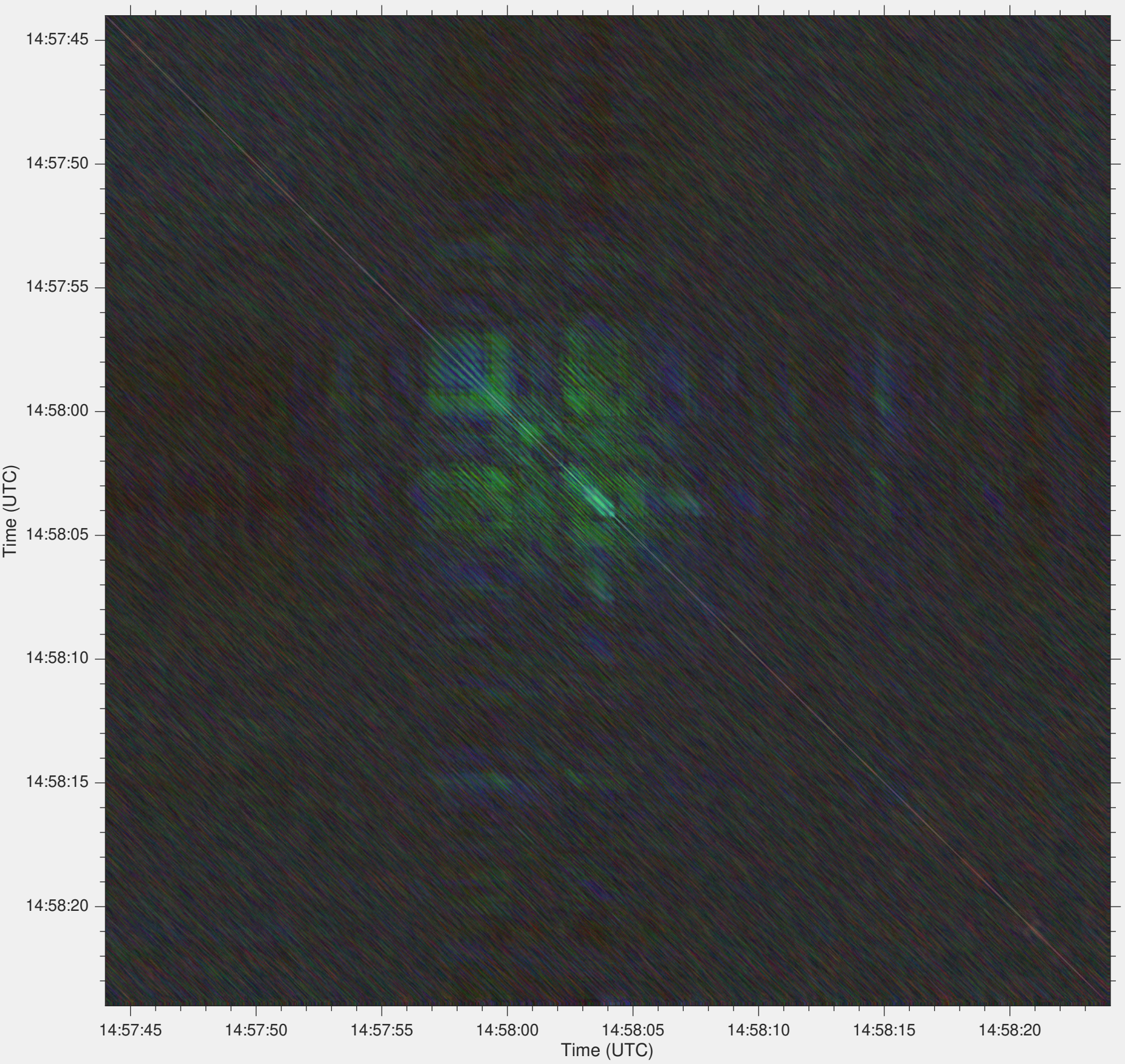
Autocorrelation plot with 200 sample window at -125 Hz H10 Nov 15 2017 14:58:04 Submarine ARA San Juan implosion
